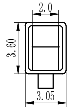
C-C SEC
