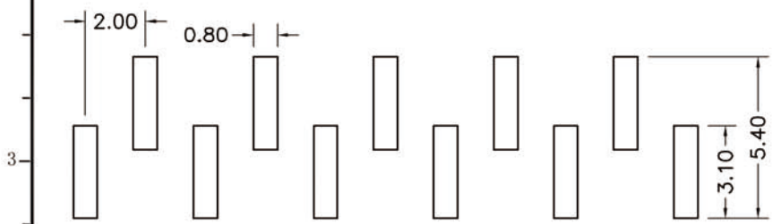
P. C. B LAYOUT
