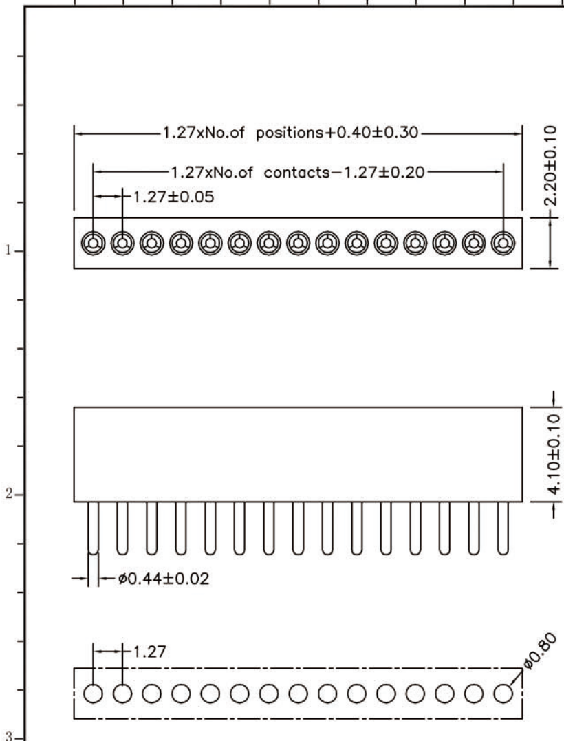
P. C. B LAYOUT
